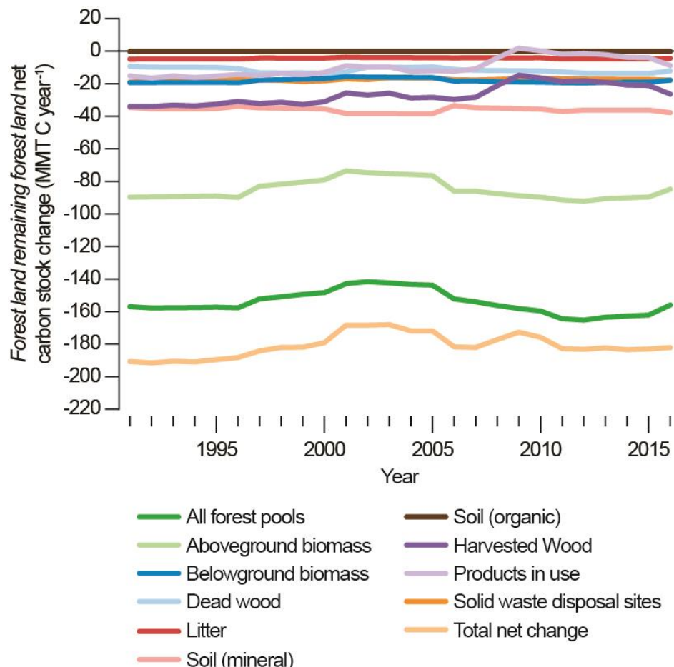
Figure 6-3: Estimated Net Annual Changes in C Stocks for All C Pools in Forest Land Remaining Forest Land in the Conterminous U.S. and Coastal Alaska (MMT C per Year)
