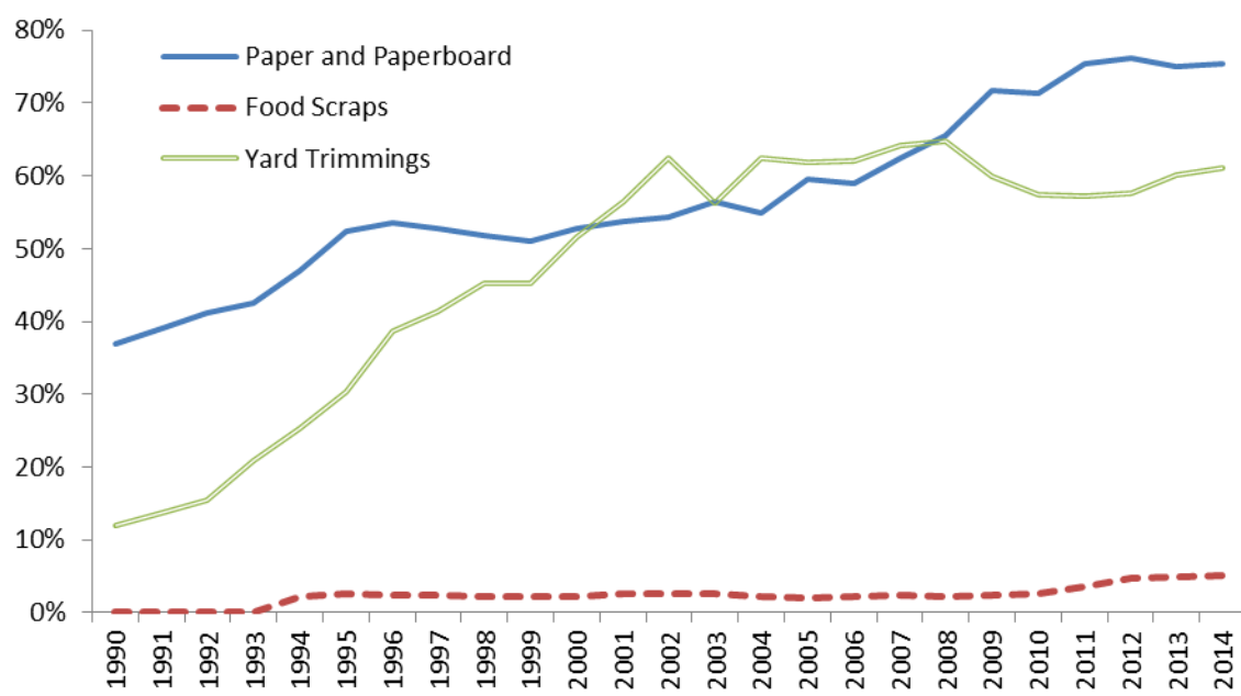
Figure 7-6: Percent of Recovered Degradable Materials from 1990 to 2014 (Percent)
