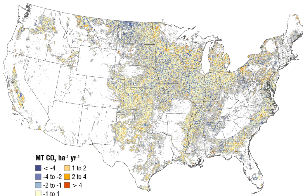
Figure 6-4: Total Net Annual CO 2 Flux for Mineral Soils under Agricultural Management within States, 2015, Cropland Remaining Cropland
