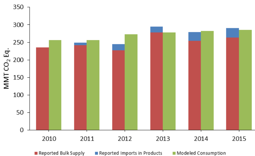
Figure 4-2: U.S. HFC Consumption (MMT CO 2 Eq.)
