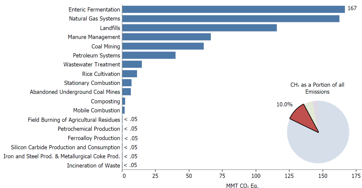
Figure ES-9: 2015 Sources of \text{CH}_4 Emissions (MMT \text{CO}_2 Eq.)
