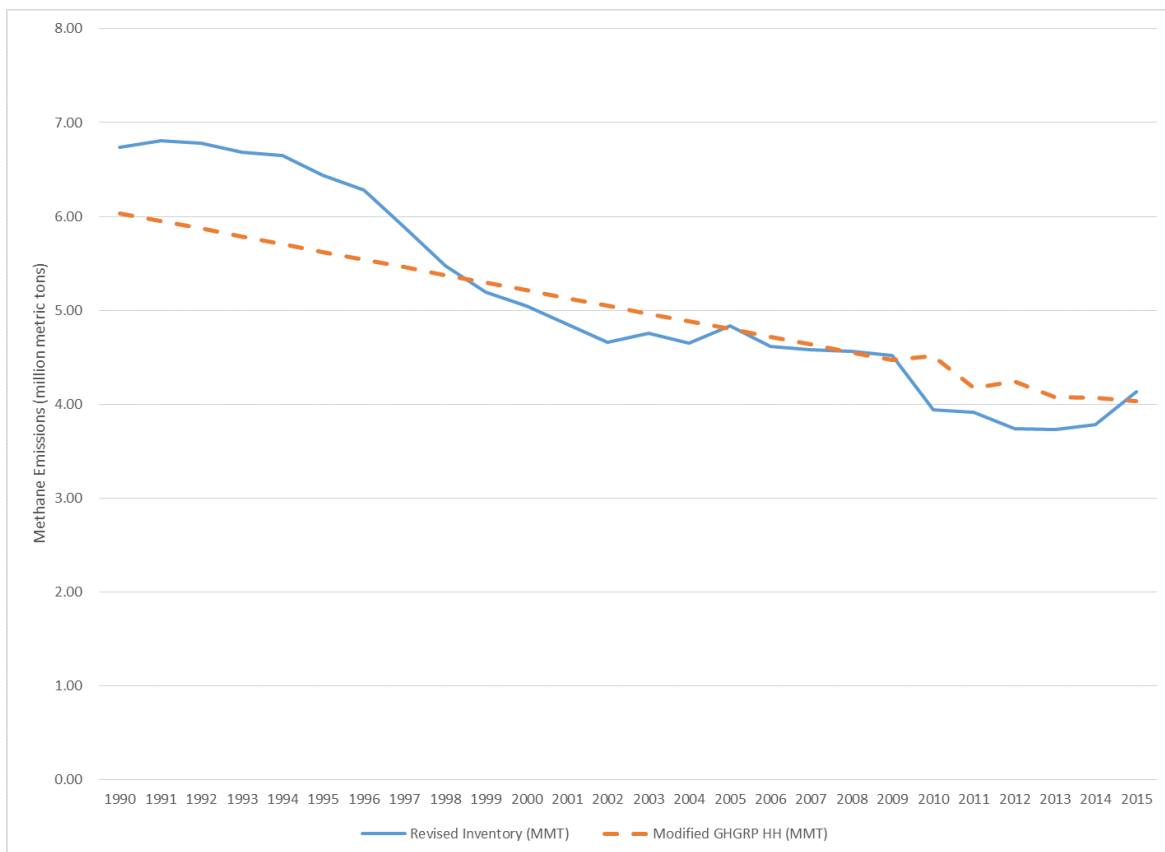
Figure 7-2: Comparison of the Revised Inventory Methodology to EPA's GHGRP Subpart HH Emissions
