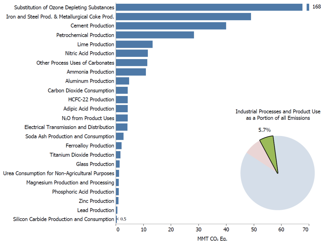
Figure 4-1: 2015 Industrial Processes and Product Use Chapter Greenhouse Gas Sources (MMT CO 2 Eq.)
