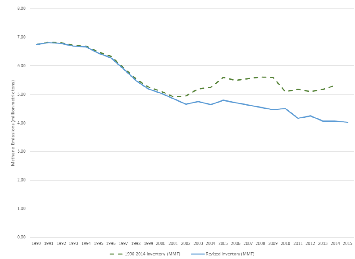
Figure 7-3: Comparison of the 1990-2014 Inventory Methodology to the Revised Inventory Methodology
