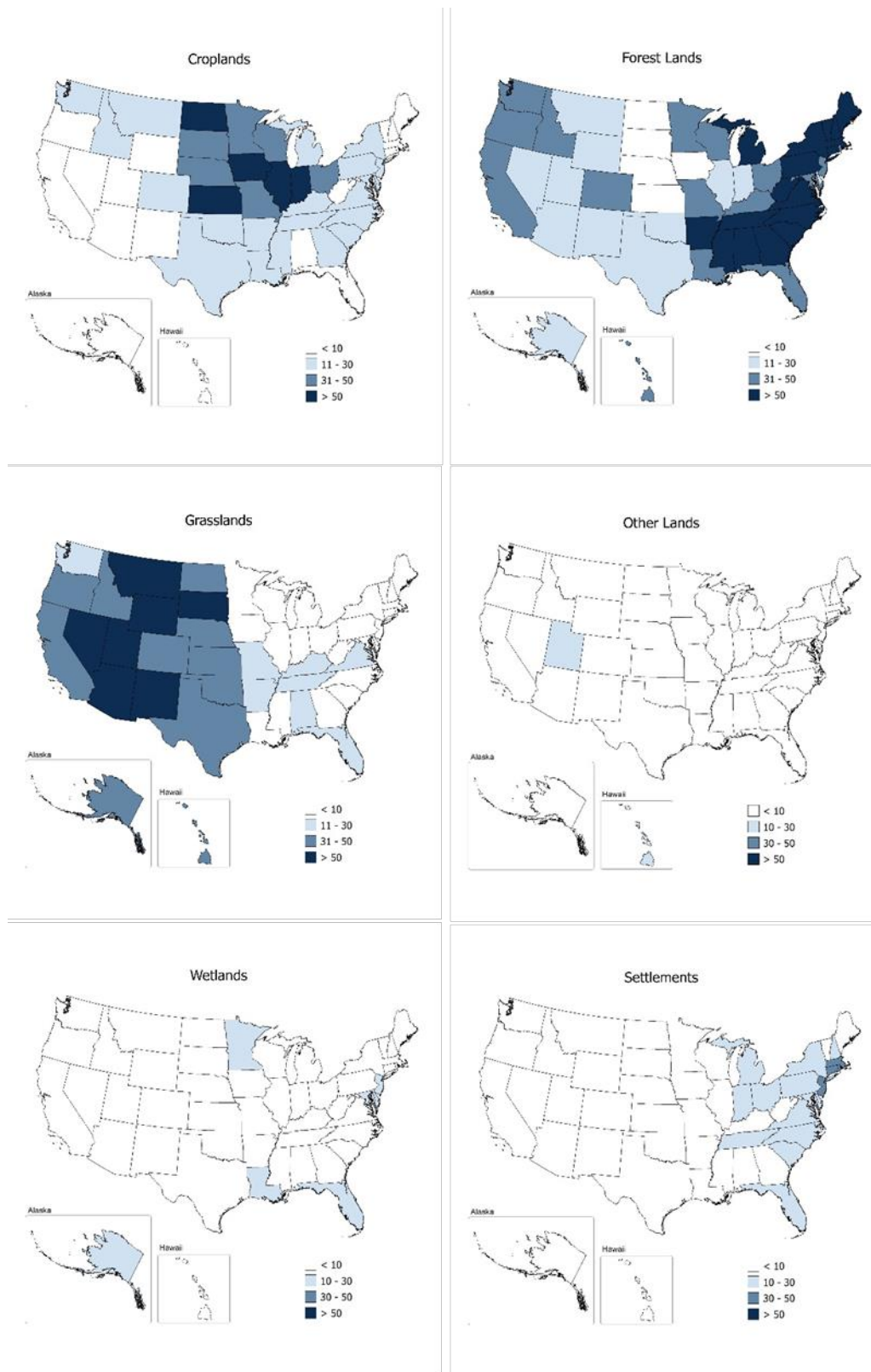
Figure 6-1: Percent of Total Land Area for Each State in the General Land-Use Categories for 2015
