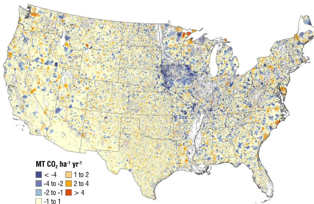
Figure 6-6: Total Net Annual CO 2 Flux for Mineral Soils under Agricultural Management within States, 2015, Grassland Remaining Grassland
